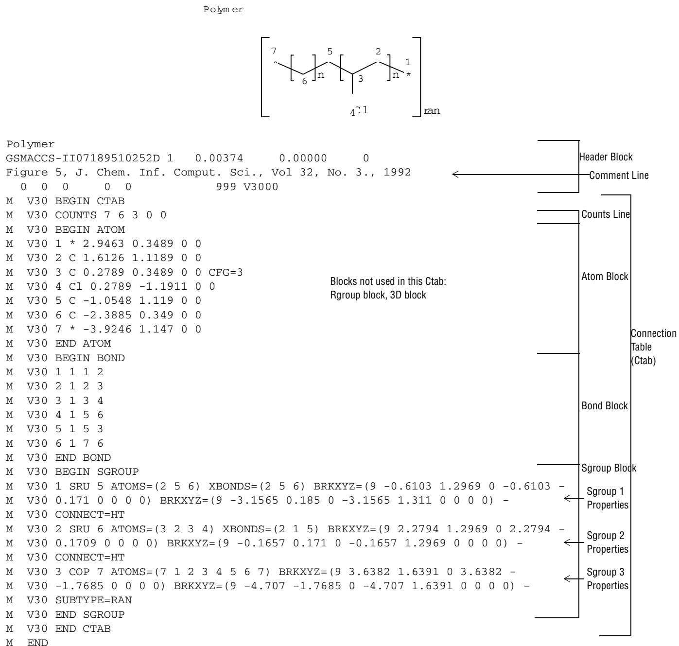
Figure 20 Connection Table Organization of an Sgroup Structure
