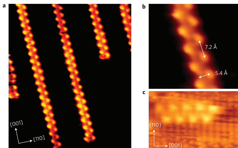
Figure 1 | Experimental STM images of water on Cu(110). a , STM image taken at 100 K showing water chains growing along the [001] direction ( 120 \times 140 \text{ \AA} , V = -196 \text{ mV} , I = -0.63 \text{ nA} ). b , Expansion of a showing partial resolution of the water structure within the chain ( 38 \times 35 \text{ \AA} ). c , Image showing protrusions residing between the Cu rows in the [001] direction ( 50 \times 30 \text{ \AA} , V = -196 \text{ mV} , I = -0.34 \text{ nA} ).
