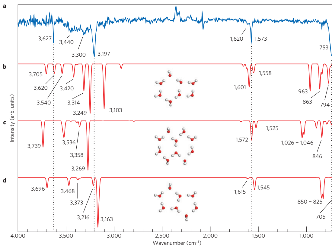
Figure 3 | Experimental and computed infrared spectra for 1D water chains on Cu(110). a , Experimental RAIRS spectrum for water chains (about 0.3 \theta_{\text{sat}} ) at 146 K. b, c , Computed infrared spectra for the hexagon-based structures shown in Fig. 2b and c, respectively. d , Computed infrared spectrum for the pentagon-based 1D chains shown in Fig. 2d.
