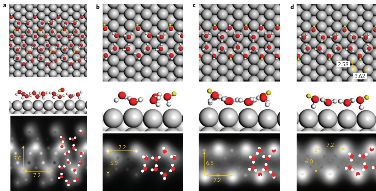
Figure 2 | Models for 1D water chains on Cu(110). a–d , Equilibrium geometry and simulated STM images for a selection of structures identified with DFT for water chains on Cu(110). Grey spheres correspond to Cu atoms, red ones to O atoms and small white ones to H atoms. The highest H atoms of each structure, which are responsible for the brightest features in the simulated STM images, are highlighted in yellow. In the simulated STM images, the locations of the water molecules in one surface unit are also shown. The most stable structure and the one we claim is observed in experiment is d , the pentagon-based structure. Distances are in Å.
